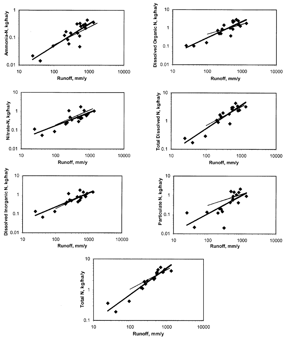
Figure 2. Relationships of runoff to total N and N fractions expressed as annual watershed yield for the 19 benchmark watersheds. The trend lines for tropical watersheds (narrow lines) from Lewis et al. (1999) are shown for comparison.
